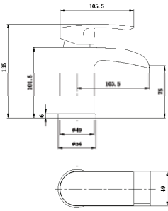
BASIN MIXER OPEN
