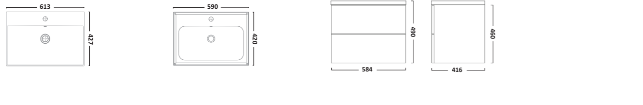
600mm Ceramic Basin 1 Tap Hole DC12012 600mm Isocast Basin 1 Tap Hole CA600IS 600mm Wall Mounted Unit Gloss White CA600W.W Gloss Light Grey CA600W.G Tundra Wood CA600W.TW Oxford Blue CA600W.OB
